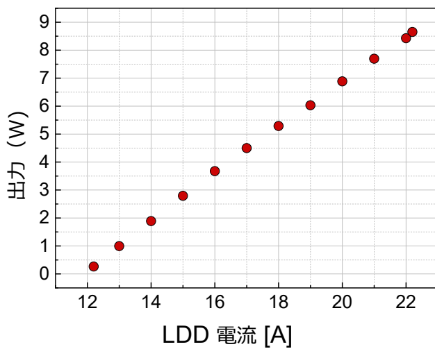
Figure 1. 1018 nm output power vs pump current
