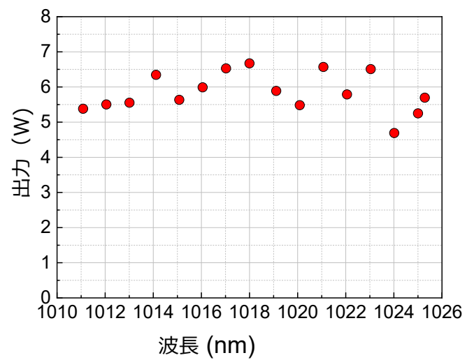
Figure 2. Tuning with birefringent filter rotation
