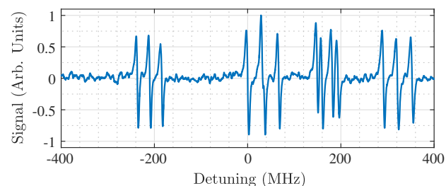
Fig. 5. Doppler-free scan of iodine lines relative to 525.4050 THz using the intracavity-doubled VC system.
