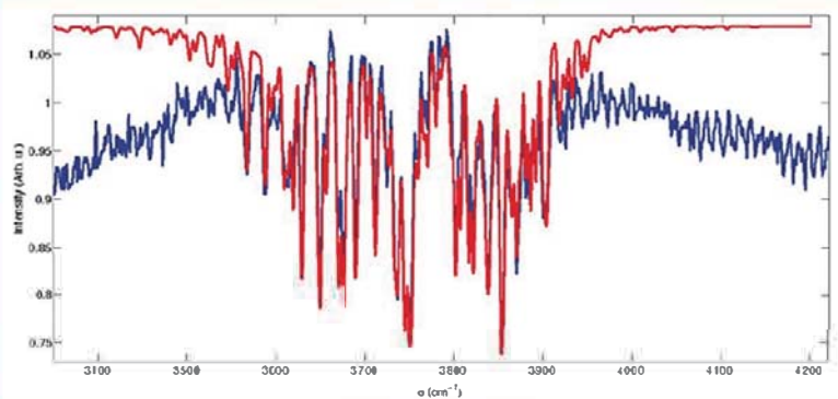
H 2 O absorption lines
