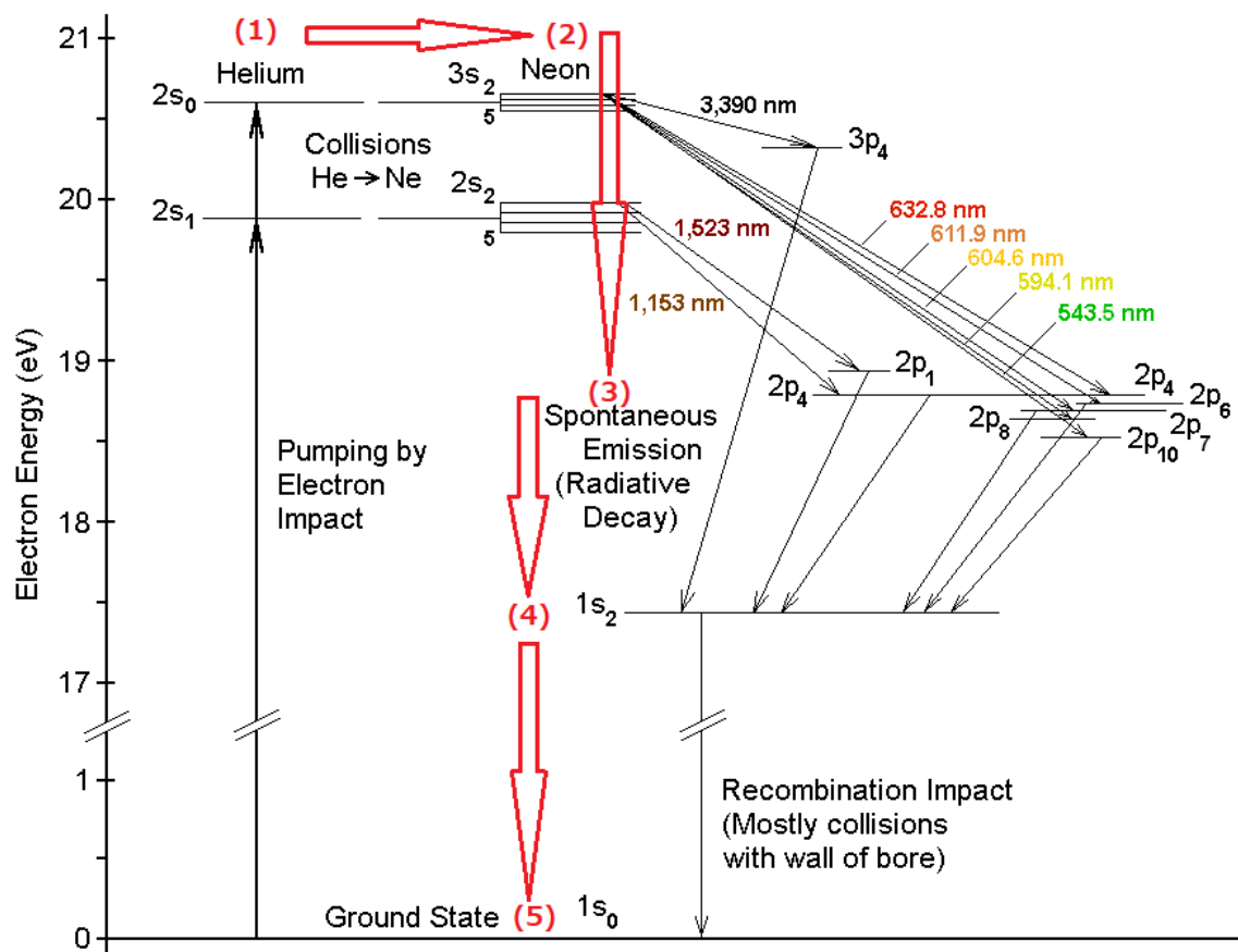
HeNe Excitation and Lasing Process
