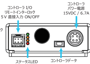
Cobolt Qu-T™ - Controller
