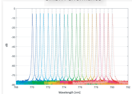
SMSR Performance
