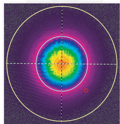
Typical Beam Profile M^2 < 1.1
