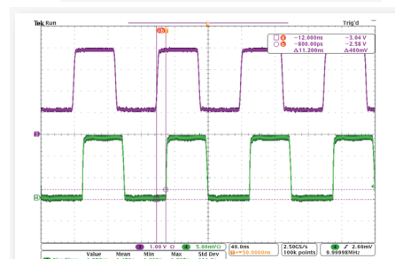
Cobolt o6- MLD Typical Digital Modulation at 10 MHz
