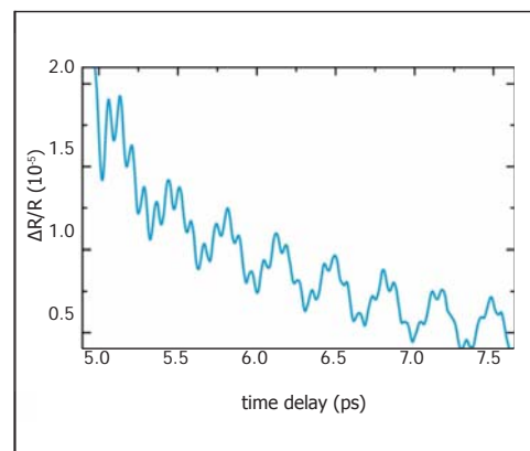
Application example: Pump-probe signature of coherent optical phonons in ZnO measured with the gecco .
